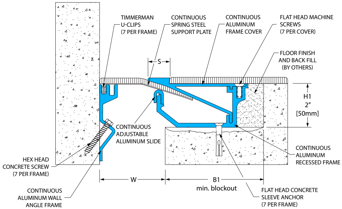
516-A02 Floor/Wall (3" (75mm) system shown)
