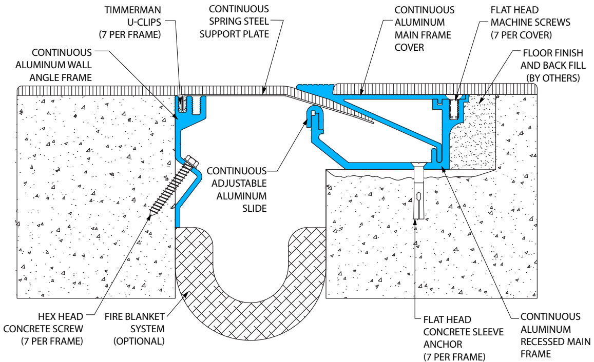
Fire Blanket System (516-A01-050 system shown)
