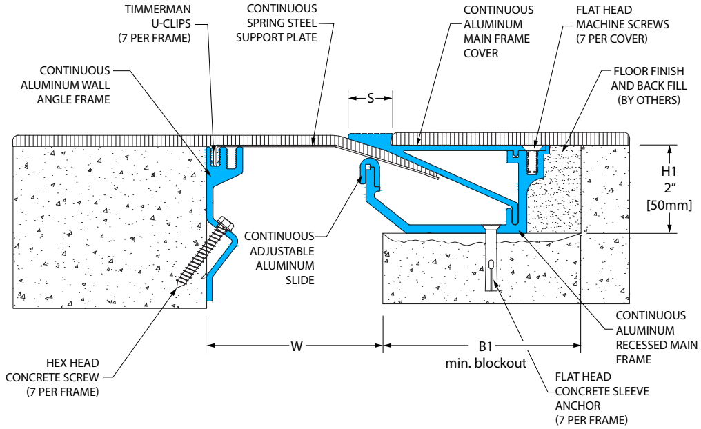
516-A01 Floor/Floor (4" (150mm) system shown)
